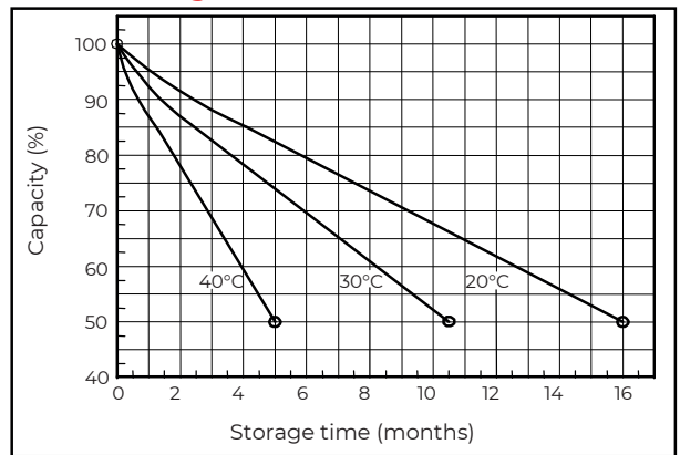
Self-discharge characteristics
